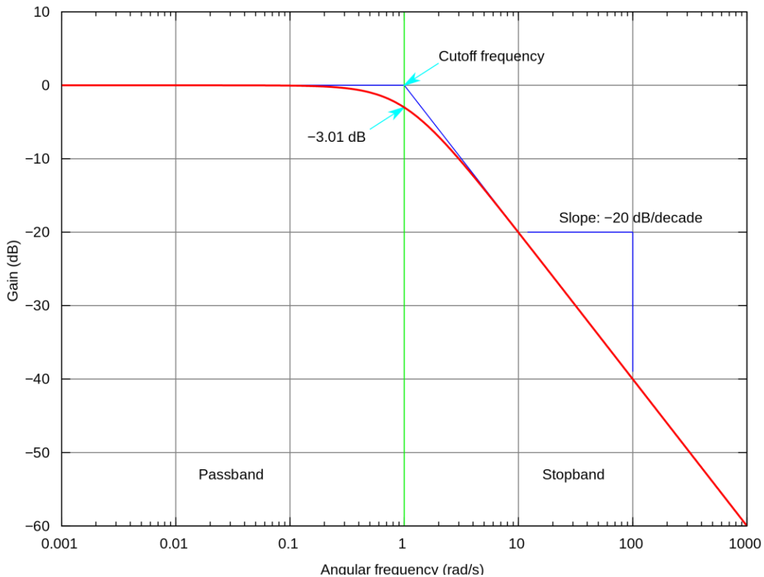
A low-pass filter frequency response chart
